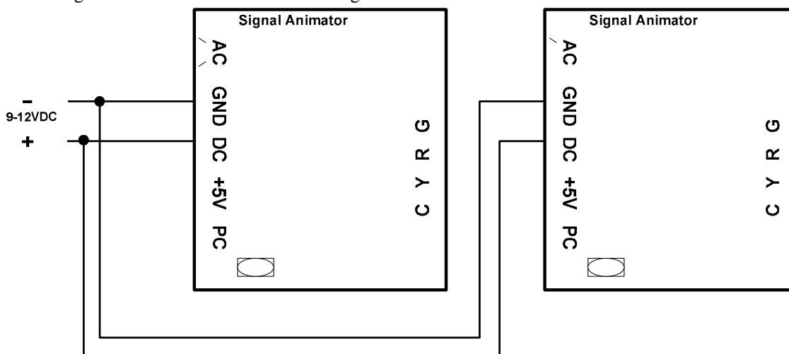
Figure 3 – DC power
