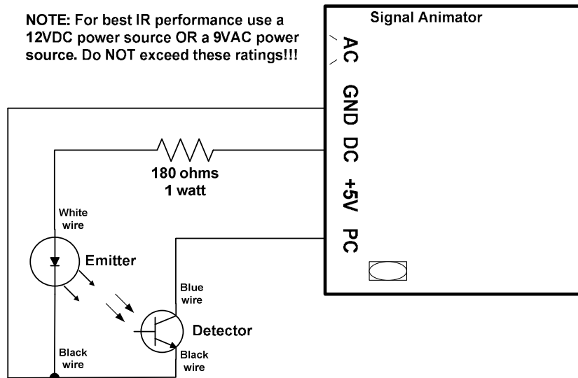
Figure 2 – IR component wiring
