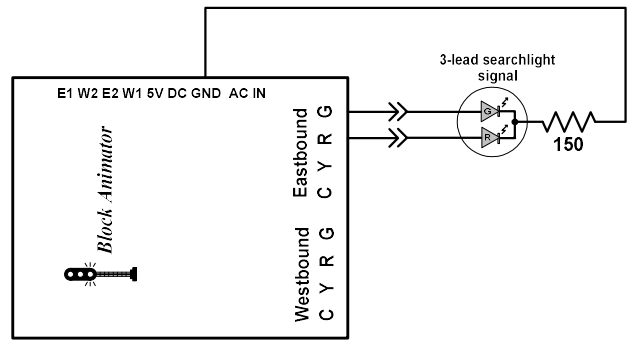
Figure 1b – three-lead bipolar
