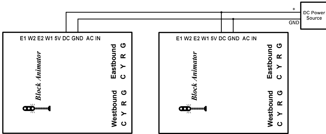
Figure 5 – DC power
