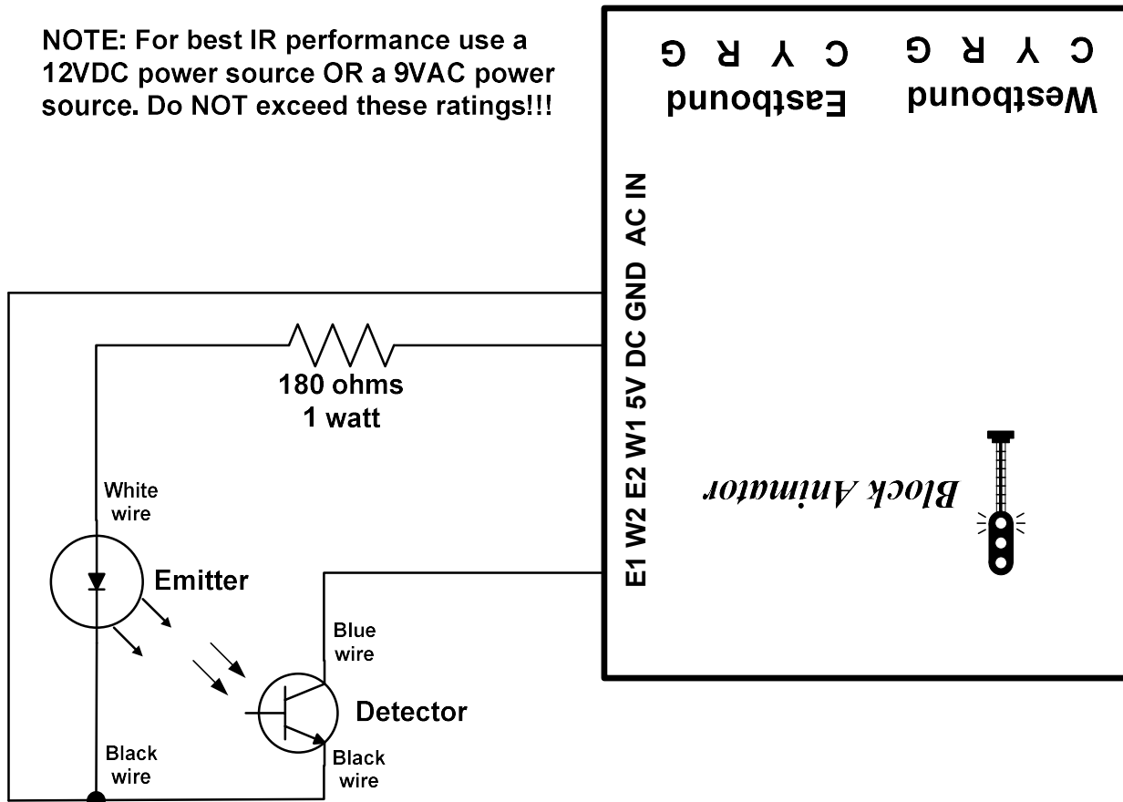
Figure 5 – IR component wiring
