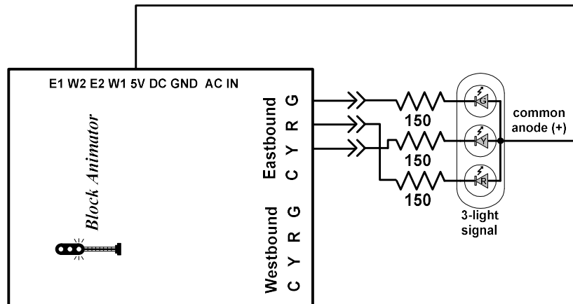
Figure 2 – 3-light signal
