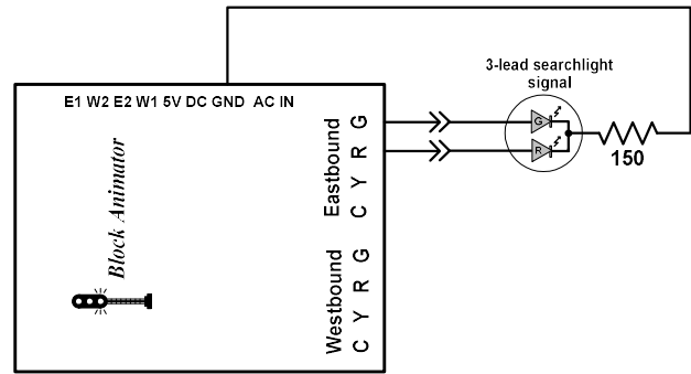
Figure 1b – three-lead searchlight signal
